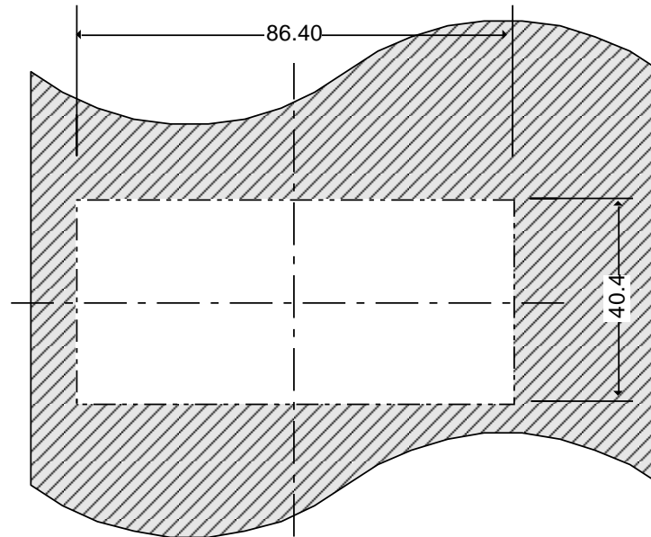
Appendix F Fig 2: Compact Door Module Mounting
